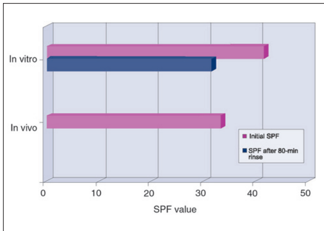
Figure 2. Water-resistant characteristics of prototype test formulation containing 1% C30-38 olefin/isopropyl maleate/MA copolymer
